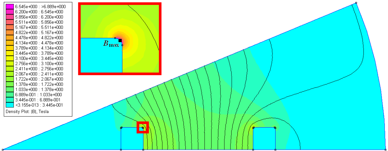
Fig. 4. Distribution of magnetic flux density and detail (2-D FEMM).
