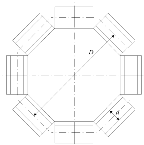
Fig. 2. Modular toroid coil cross section [11].
