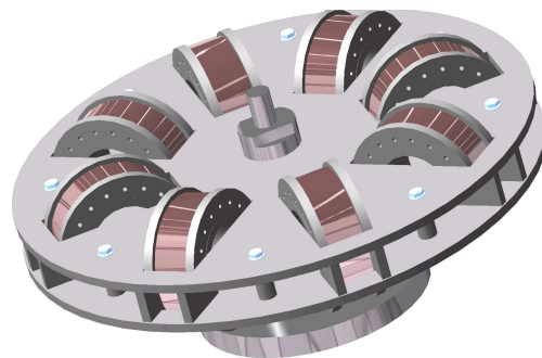
Fig. 1. Modular toroid coil 3-D view.
