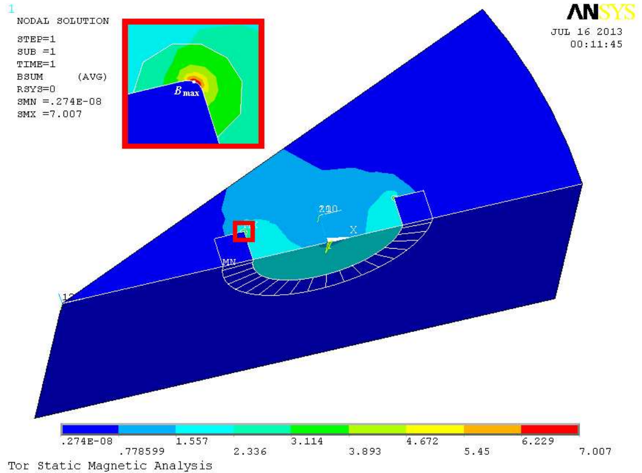
Fig. 5. Distribution of magnetic flux density and detail (3-D ANSYS).
